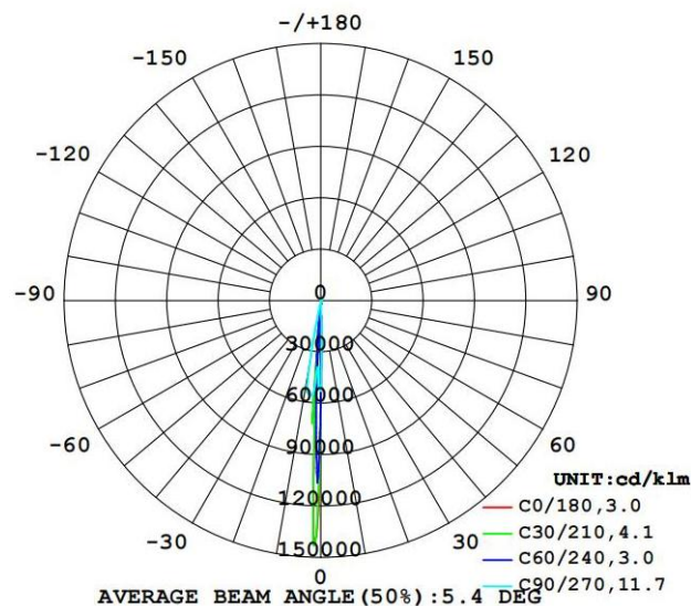
Lighting Distribution
